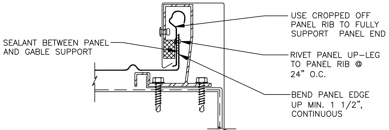
ALTERNATE DETAIL PANEL ENDS OFF MODULE
