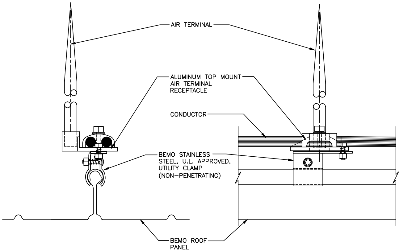
LIGHTNING PROTECTION ATTACHMENT TO BEMO ROOF PANELS.
