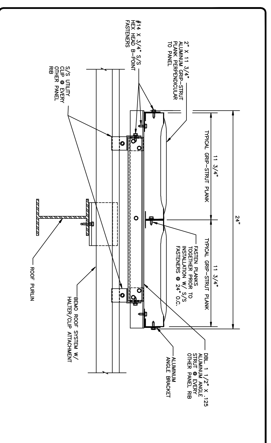
PANEL: BEMO 400 DETAIL: GRIP STRUT SAFETY GRATING, PERPENDICULAR TO PANEL DATE: 09/11/02 PAGE: 1 OF 1
