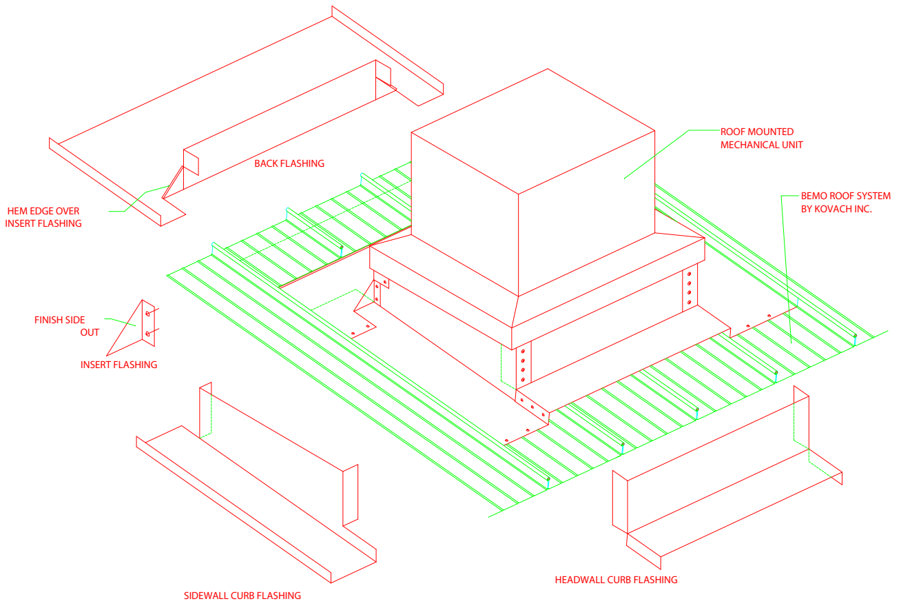
BEMO ROOF CURB DETAIL
